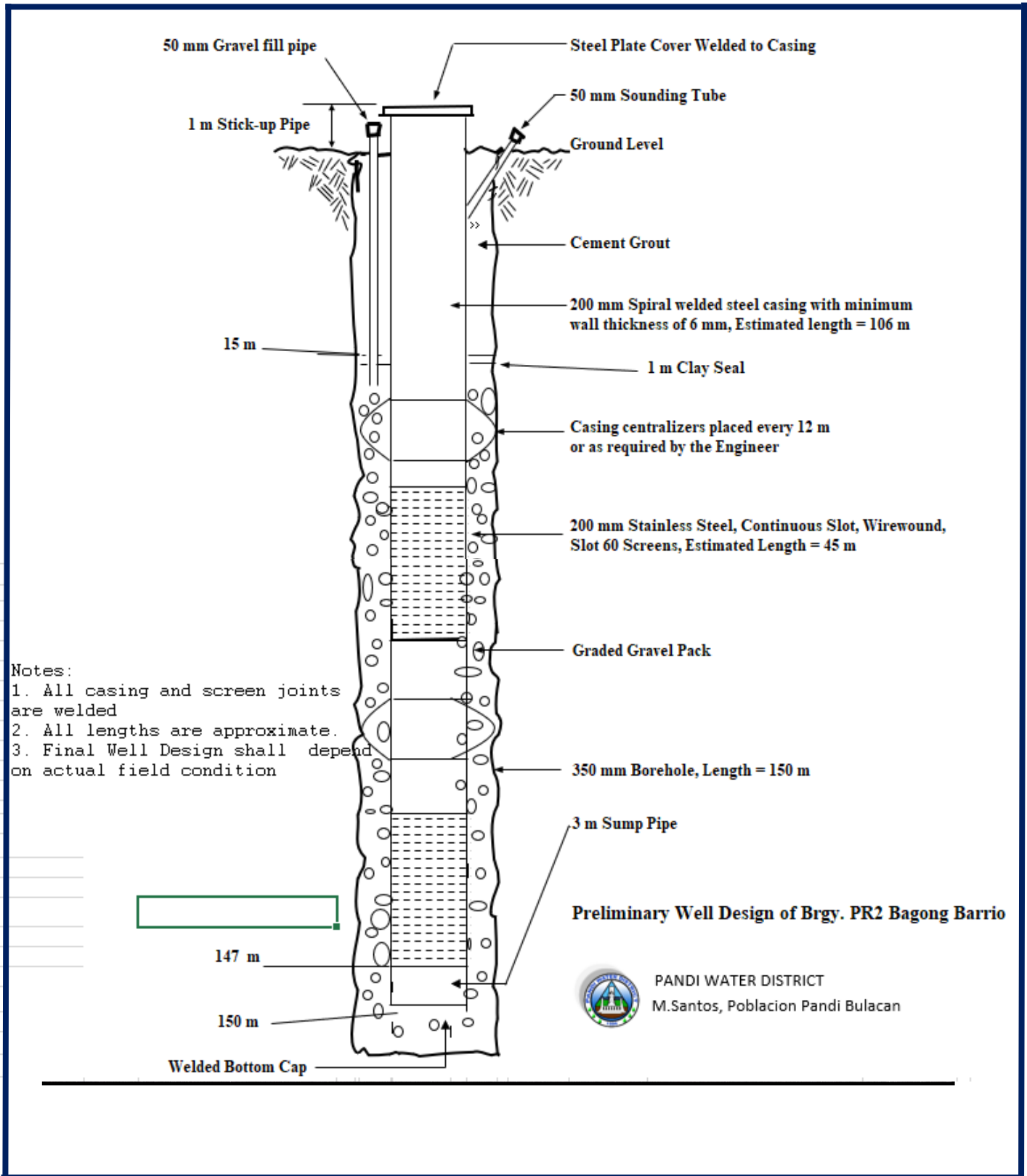
Well Design
