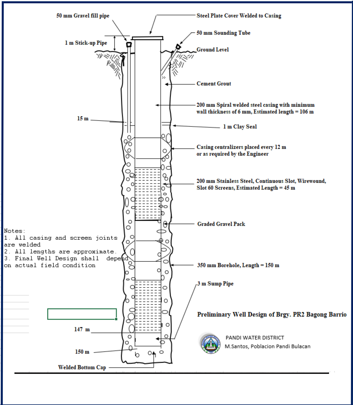
Well Design
